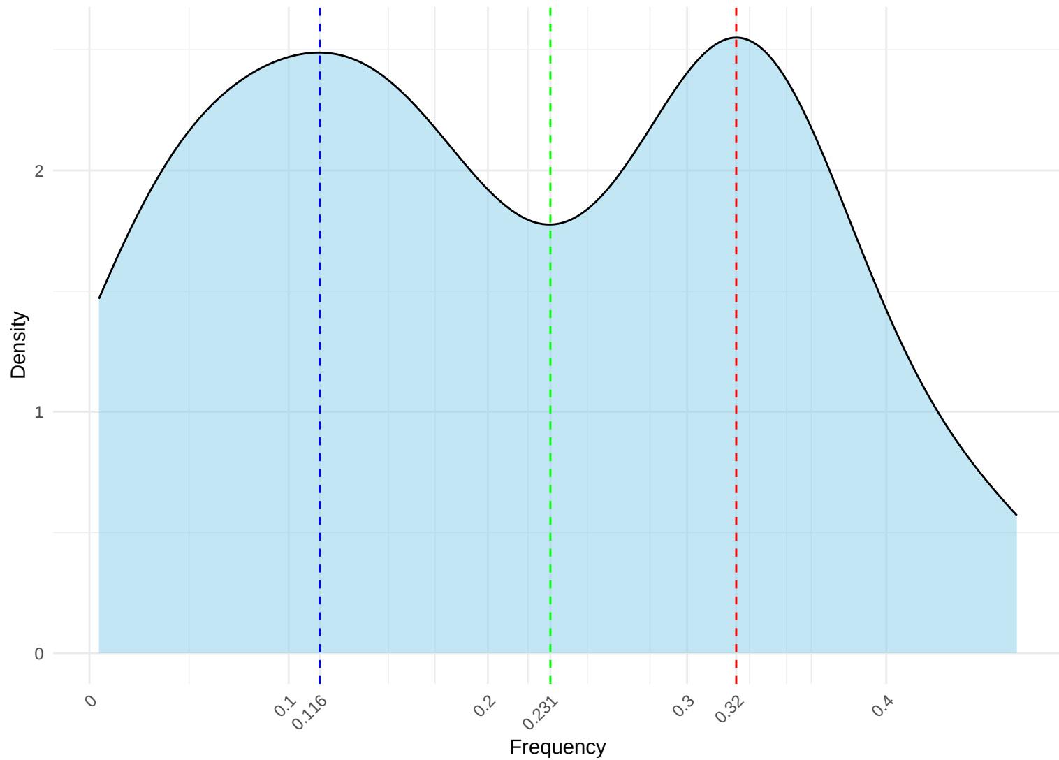
chimpanzee – exitron Distribution
