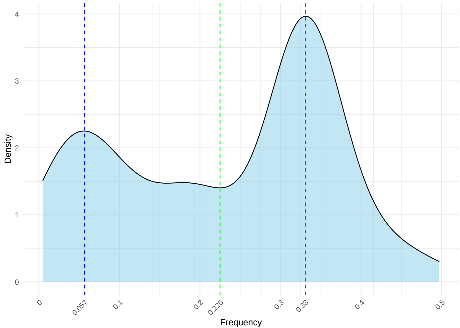
gibbon – exitron Distribution
