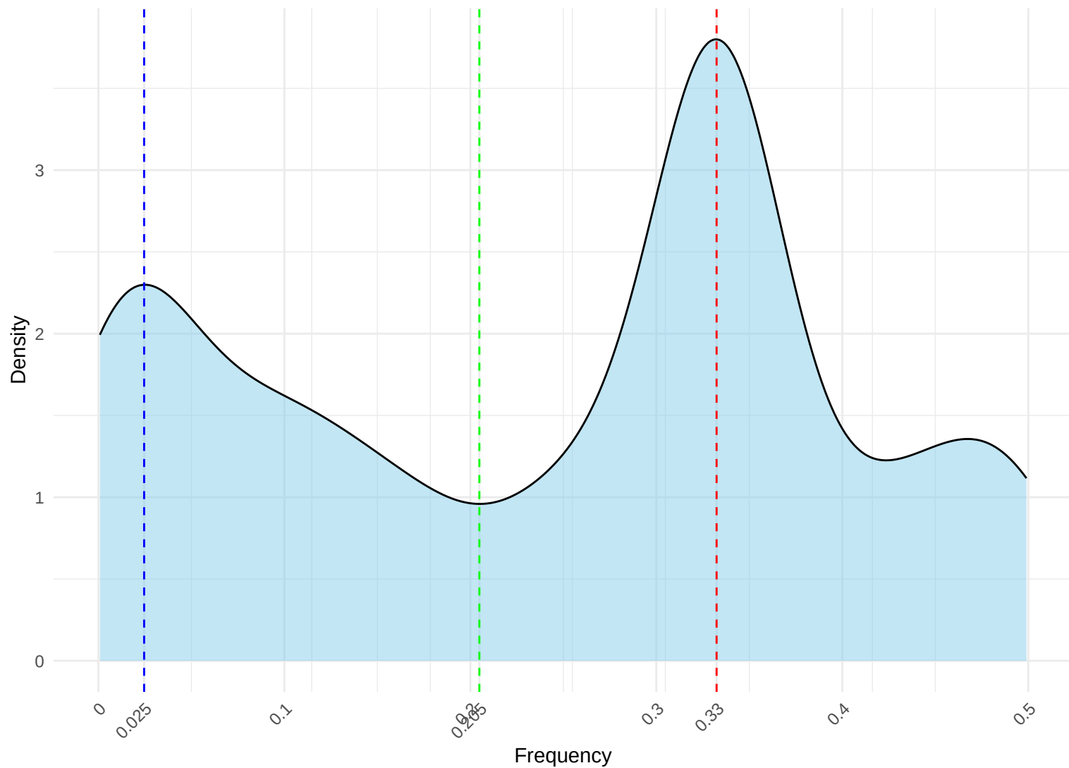
gibbon – upstream Distribution
