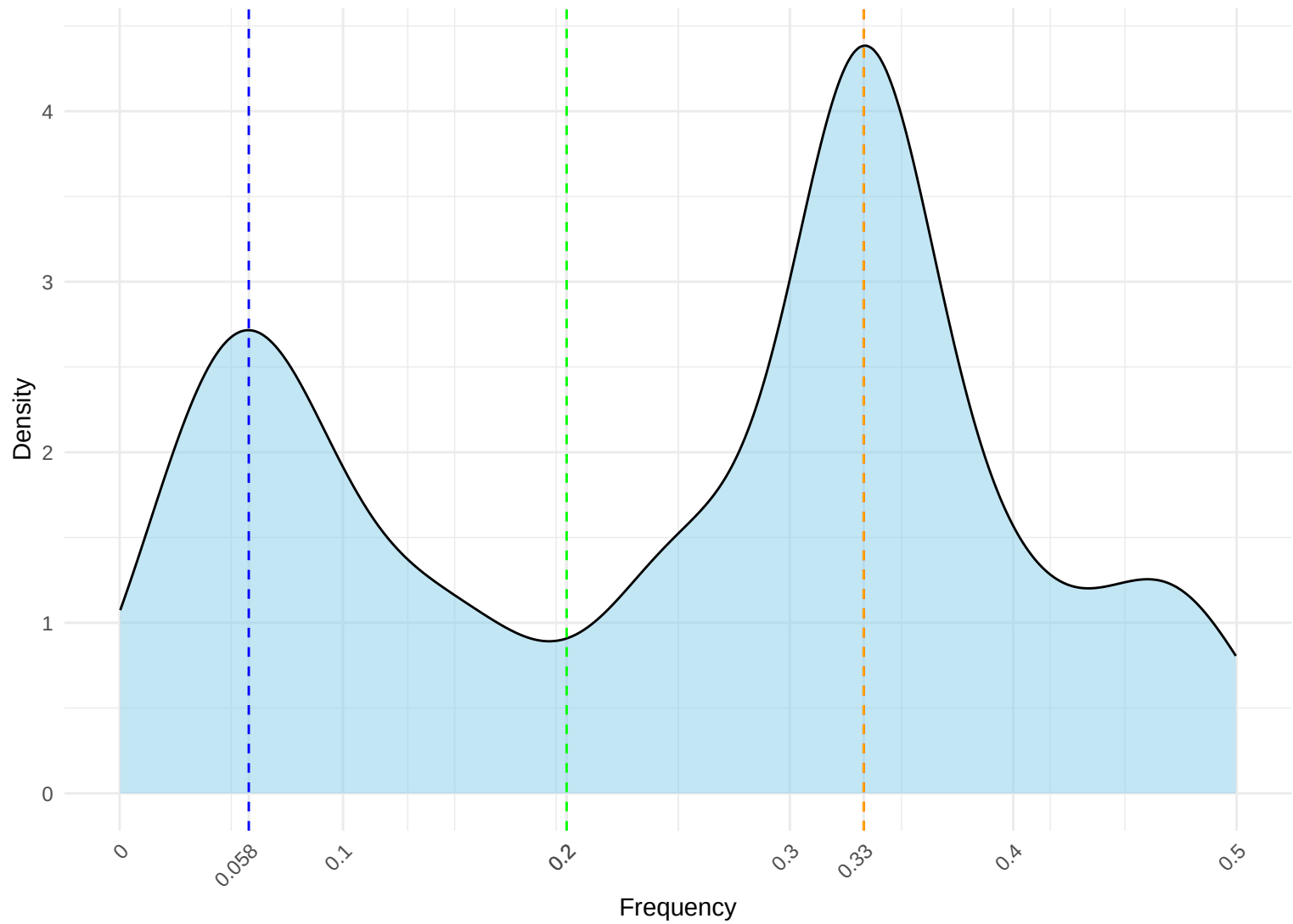
human – SCFR Distribution
