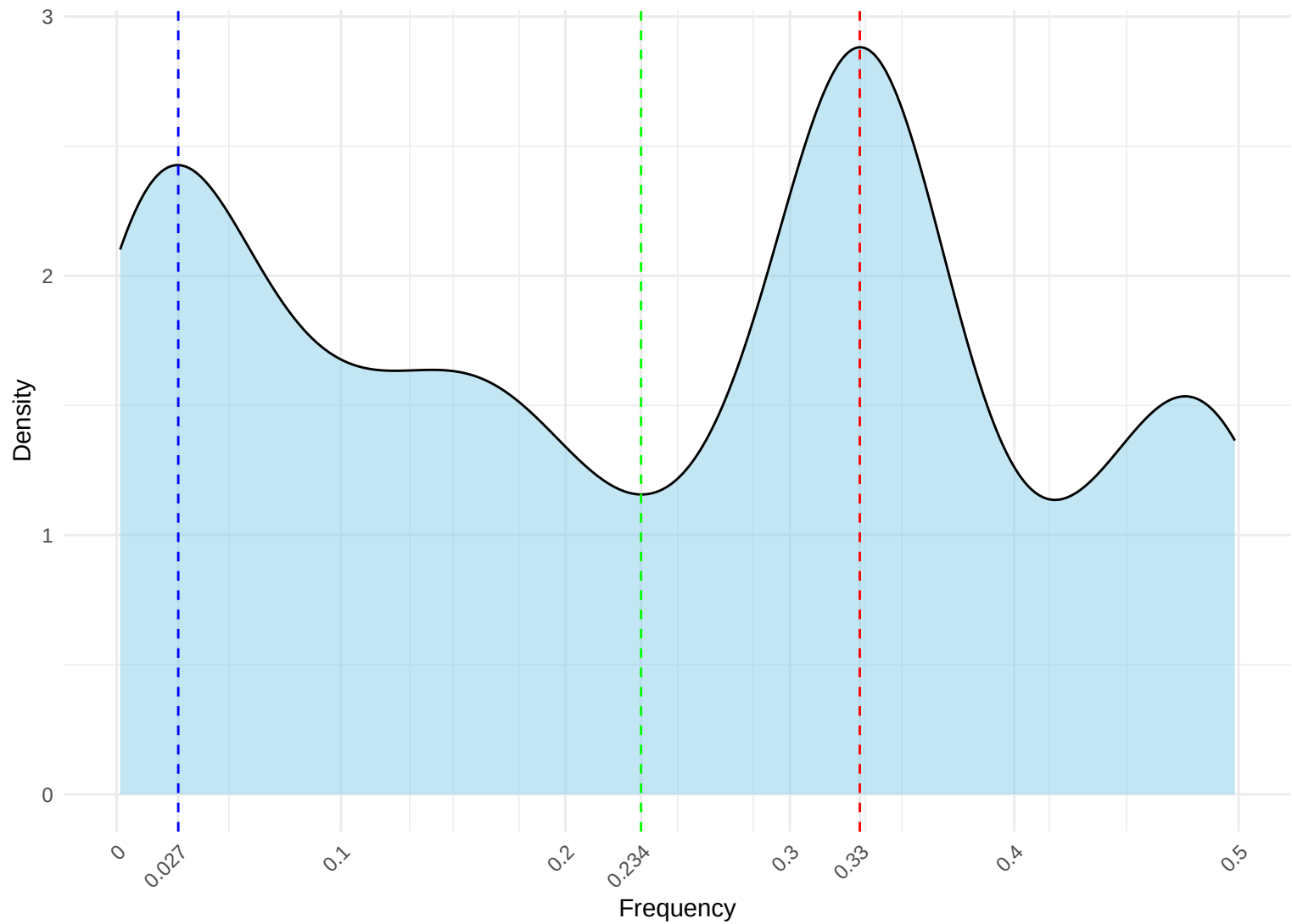
human – upstream Distribution
