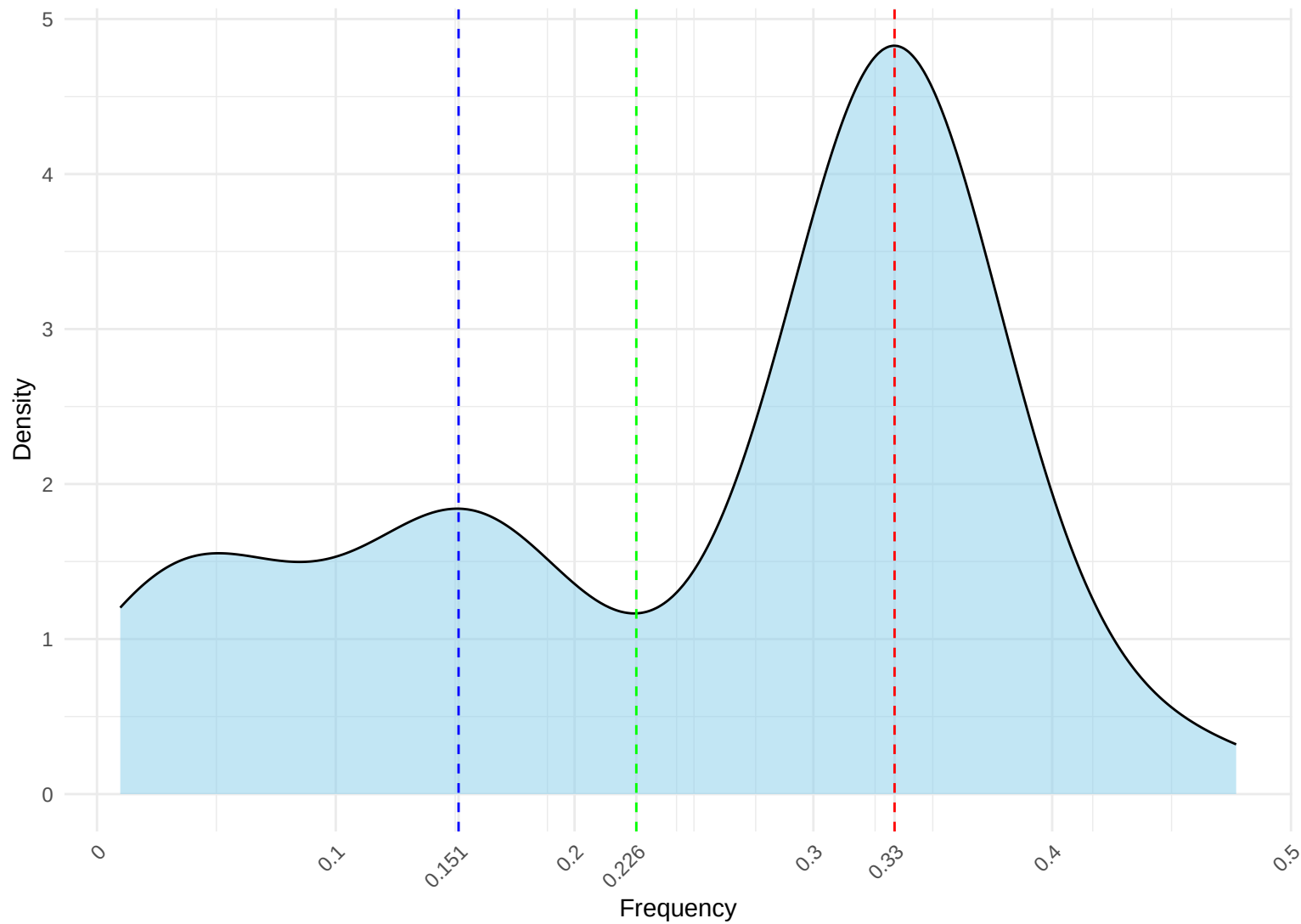
sorangutan – exitron Distribution
