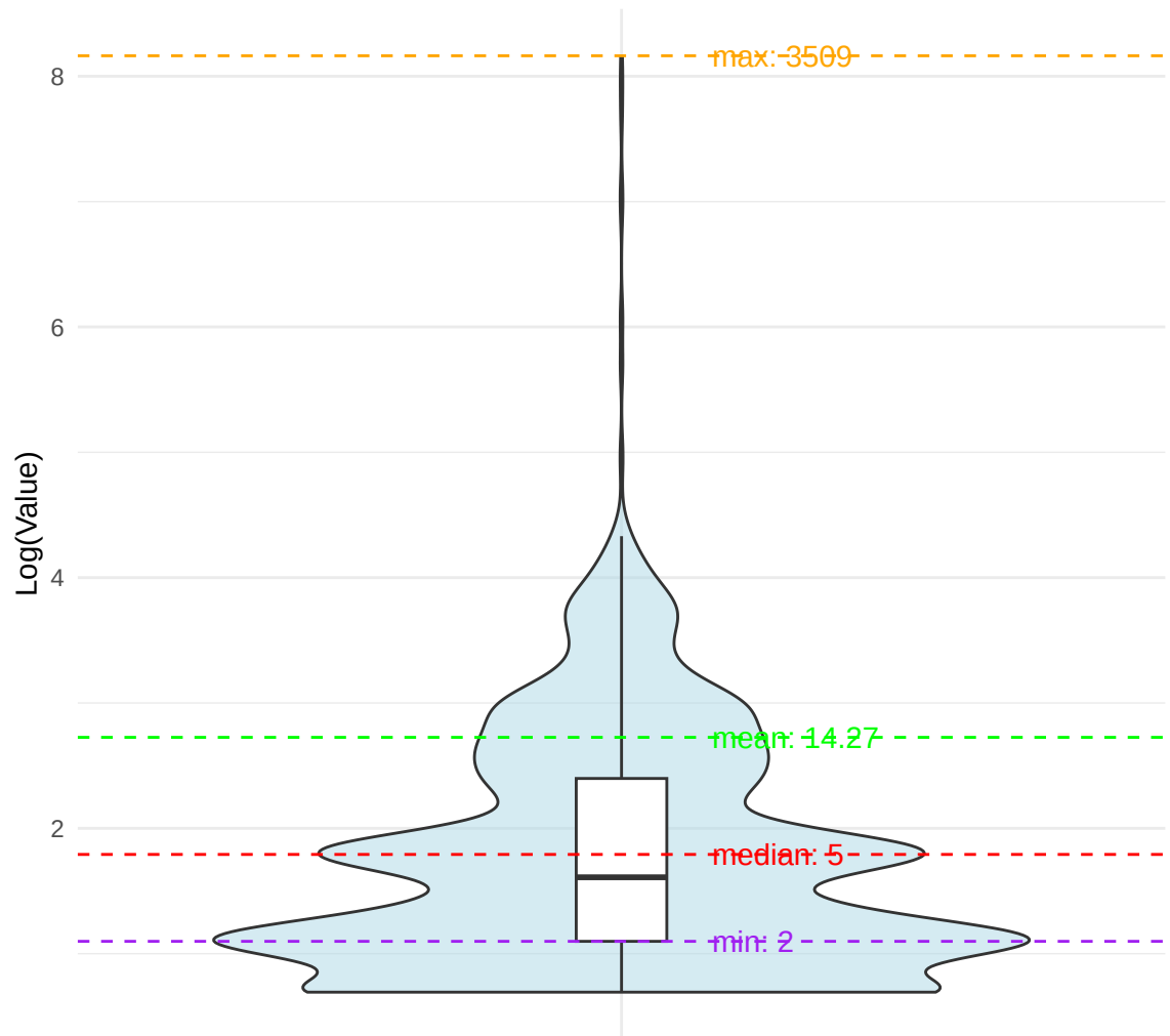
bonobo – SCFR Violin Plot
