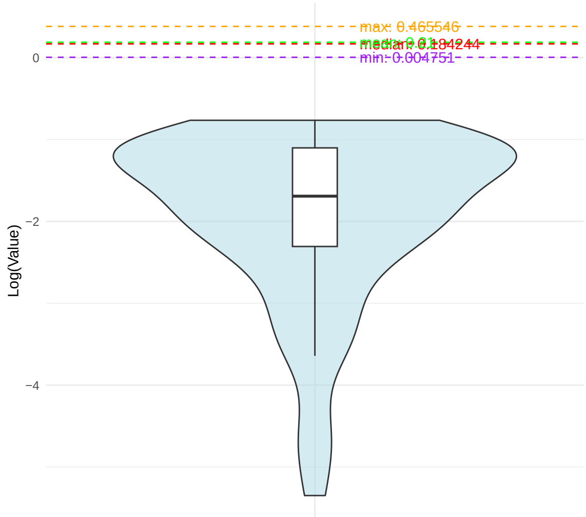
chimpanzee – exon Violin Plot
