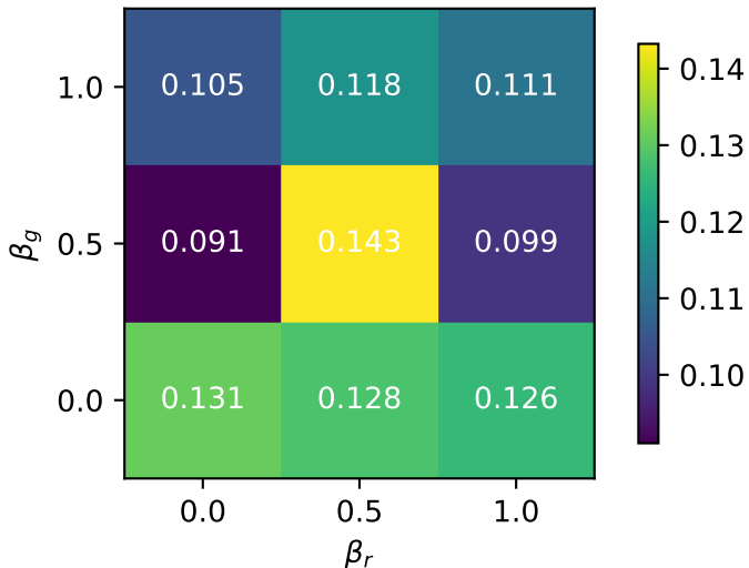
Beta Sweep
