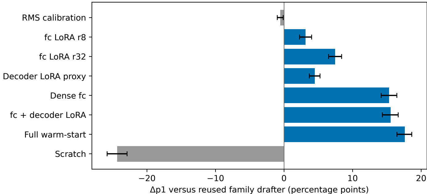
R1-Distill-Llama: 256 self-elicited examples, seed 0 Trained: 300 steps; RMS: training-free; SPEED-128 paired 95% intervals
