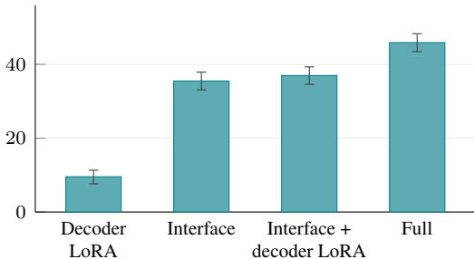
Dedicated-drafter gap recovered (%)
