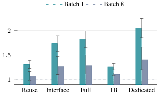
R1-Distill-Llama-8B
