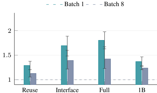
Nemotron-Nano-8B
