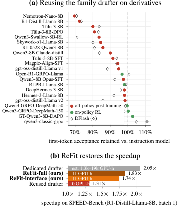
Figure 1: (a) First-token acceptance of the production family drafters (EAGLE-3 dots, DFlash diamonds) on 21 widely used Llama-3.1-8B and Qwen3-8B derivatives, relative to the instruction model they were trained for, on the same 128 SPEED-Bench prompts. On-policy RL leaves the drafter intact; off-policy post-training can break it, most severely in the extensively post-trained reasoning models at the top. The 174-derivative census is in Appendix E. (b) On R1-Distill-Llama-8B, ReFit recovers most of the speedup of a dedicated drafter at a small fraction of its training cost.
