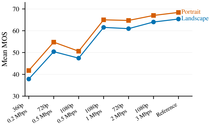
(a) Portrait video scores higher at every rung
