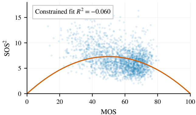
(b) The standard SOS relation does not fit
