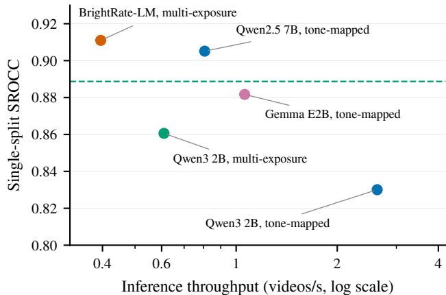
(b) Accuracy versus throughput
