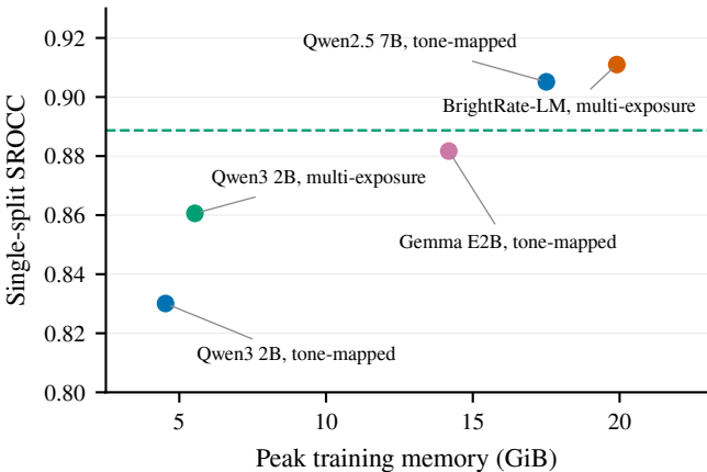
(a) Accuracy versus memory
