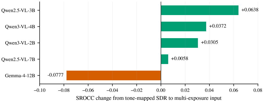
Multi-exposure input improves four of five models
