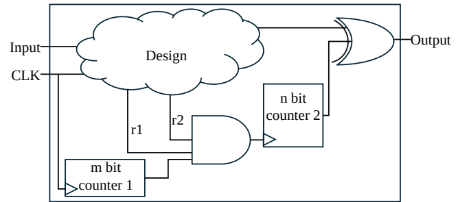
FIGURE 4: A sample Trojan from our experiment that applies a hybrid trigger mechanism.
