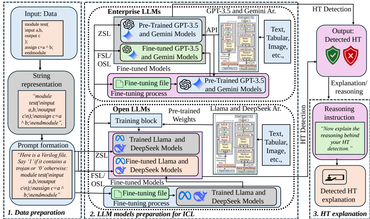
FIGURE 1: Our proposed HT detection and explanation framework, where architecture denoted as (Ar.)
