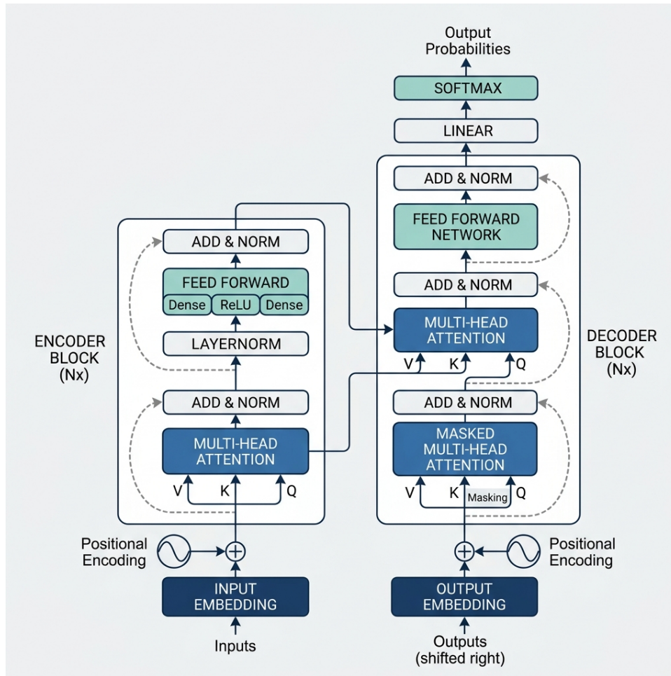
Figure 2.1: The general architecture of the Transformer model, showcasing the encoder-decoder structure, multi-head self-attention, positional encoding, and feed-forward networks.
