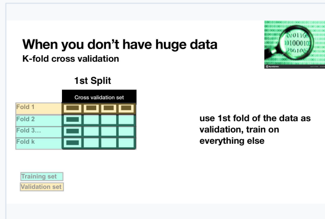
K-fold cross-validation
