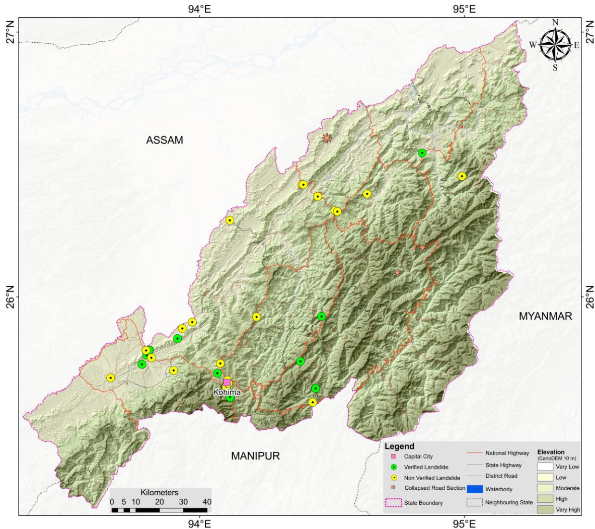
Map 7 Landslide incidents in Nagaland, 2025
