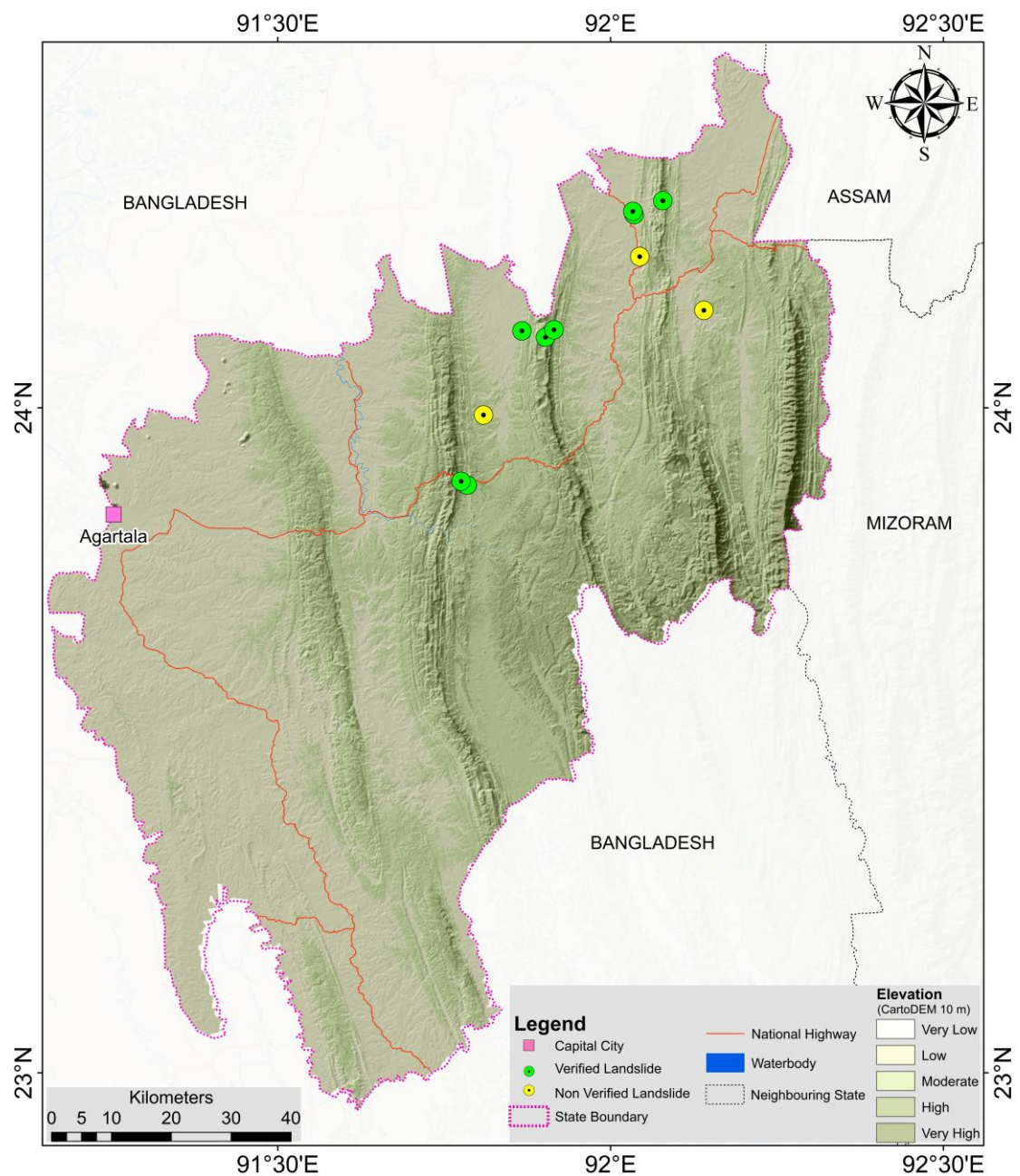
Map 9 Landslide incidents in Tripura, 2025
