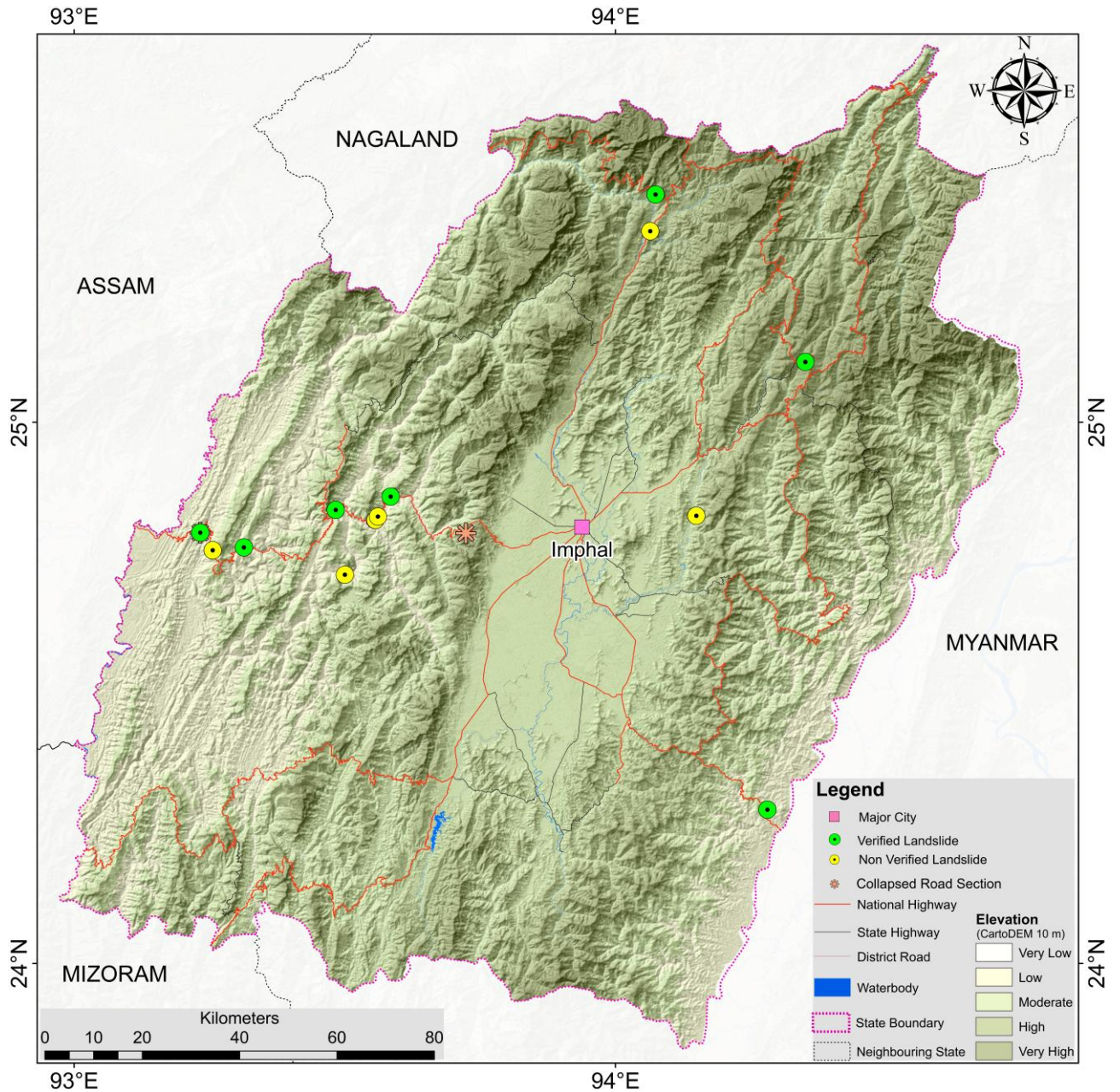
Map 4 Landslide incidents in Manipur, 2025
