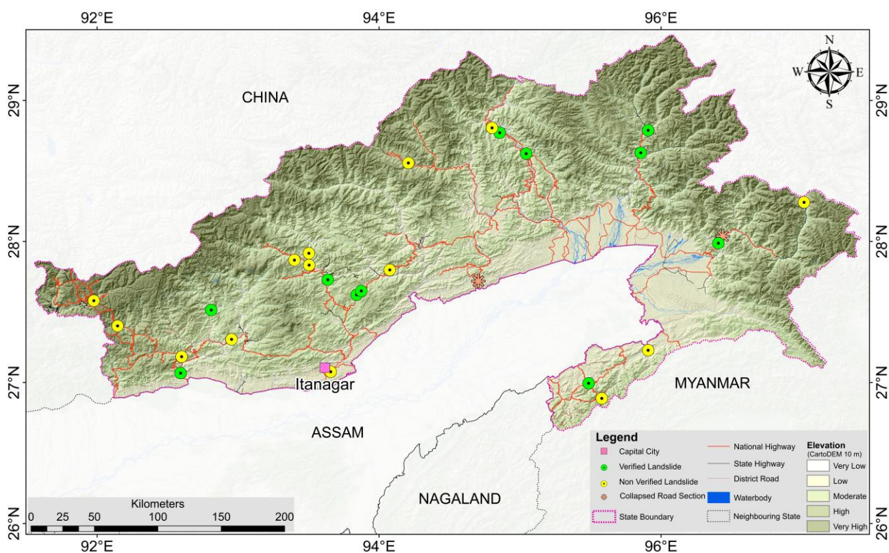
Map 2 Landslide incidents in Arunachal Pradesh, 2025
