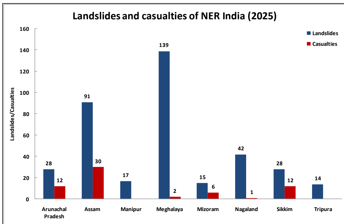
Figure 3 Landslides and casualties of NER, India in 2025
