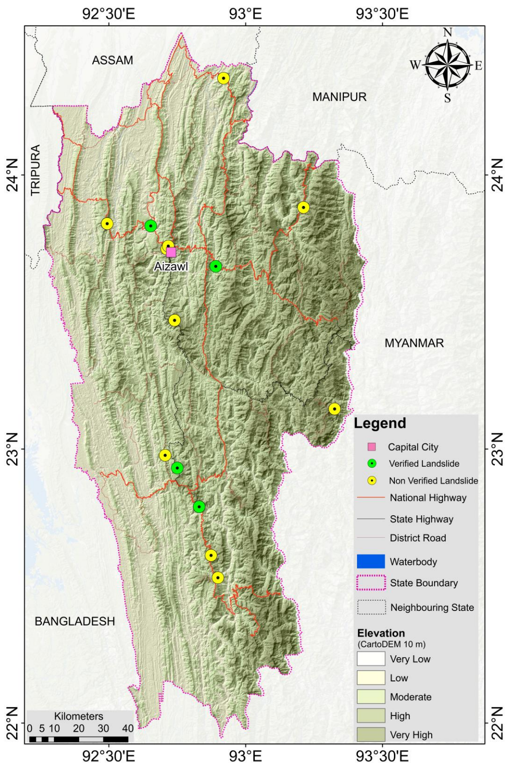
Map 6 Landslide incidents in Mizoram, 2025
