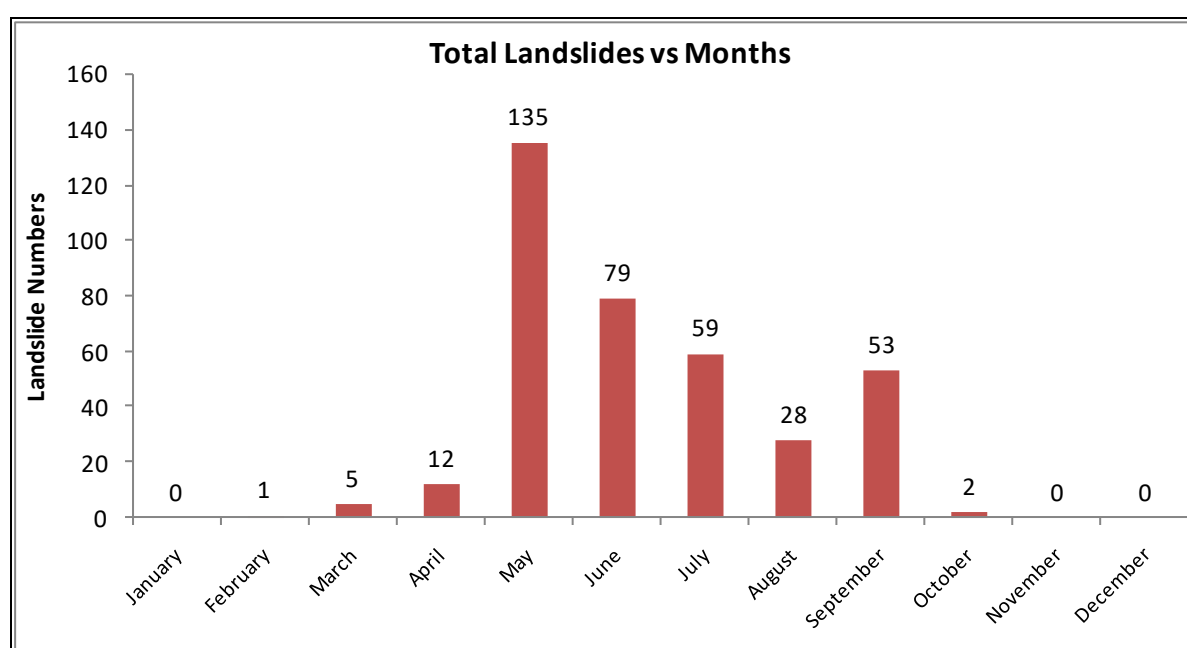
Figure 4 Monthwise landslides in NER, India (2025)
