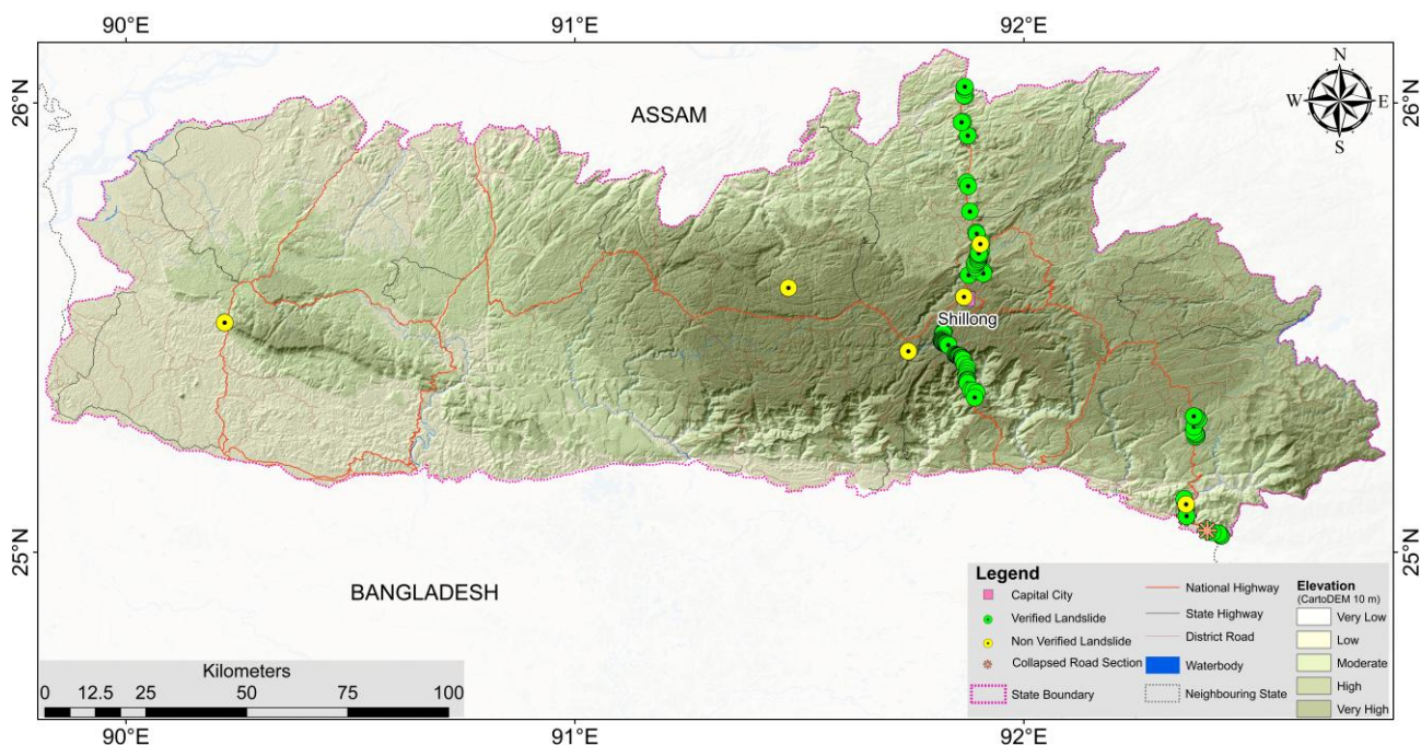
Map 5 Landslide incidents in Meghalaya, 2025
