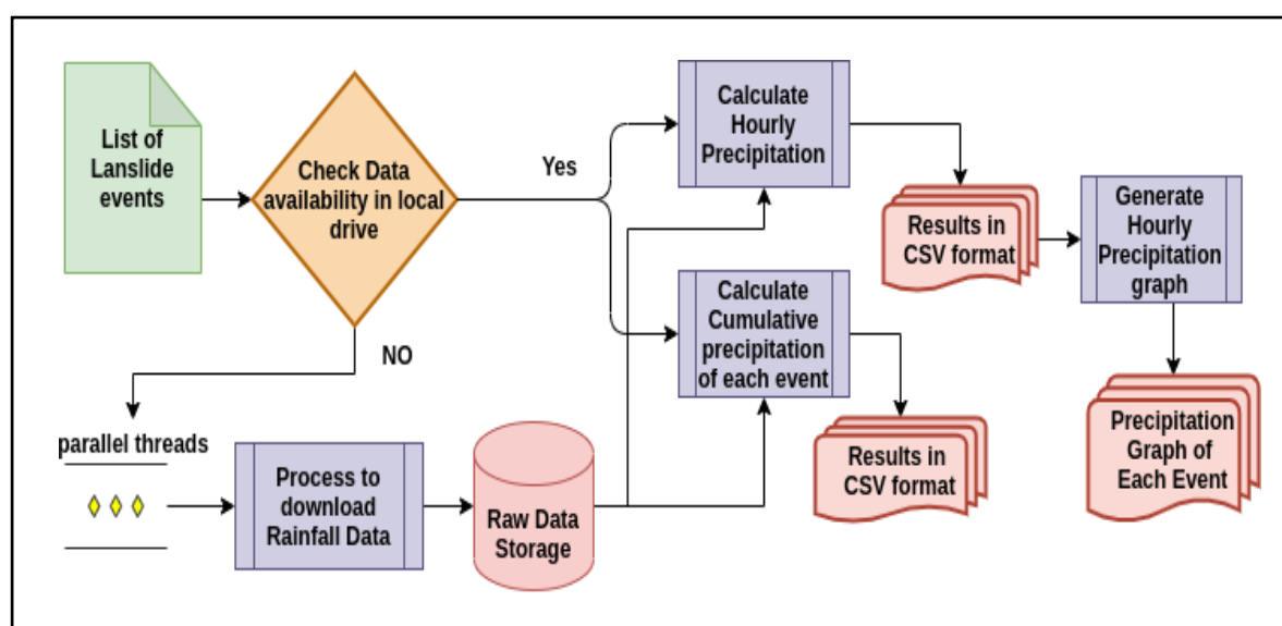
Figure 2 Flowchart for automatic extraction of rainfall
