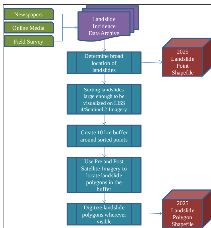
Figure 1 Flowchart of Landslide polygon extraction
