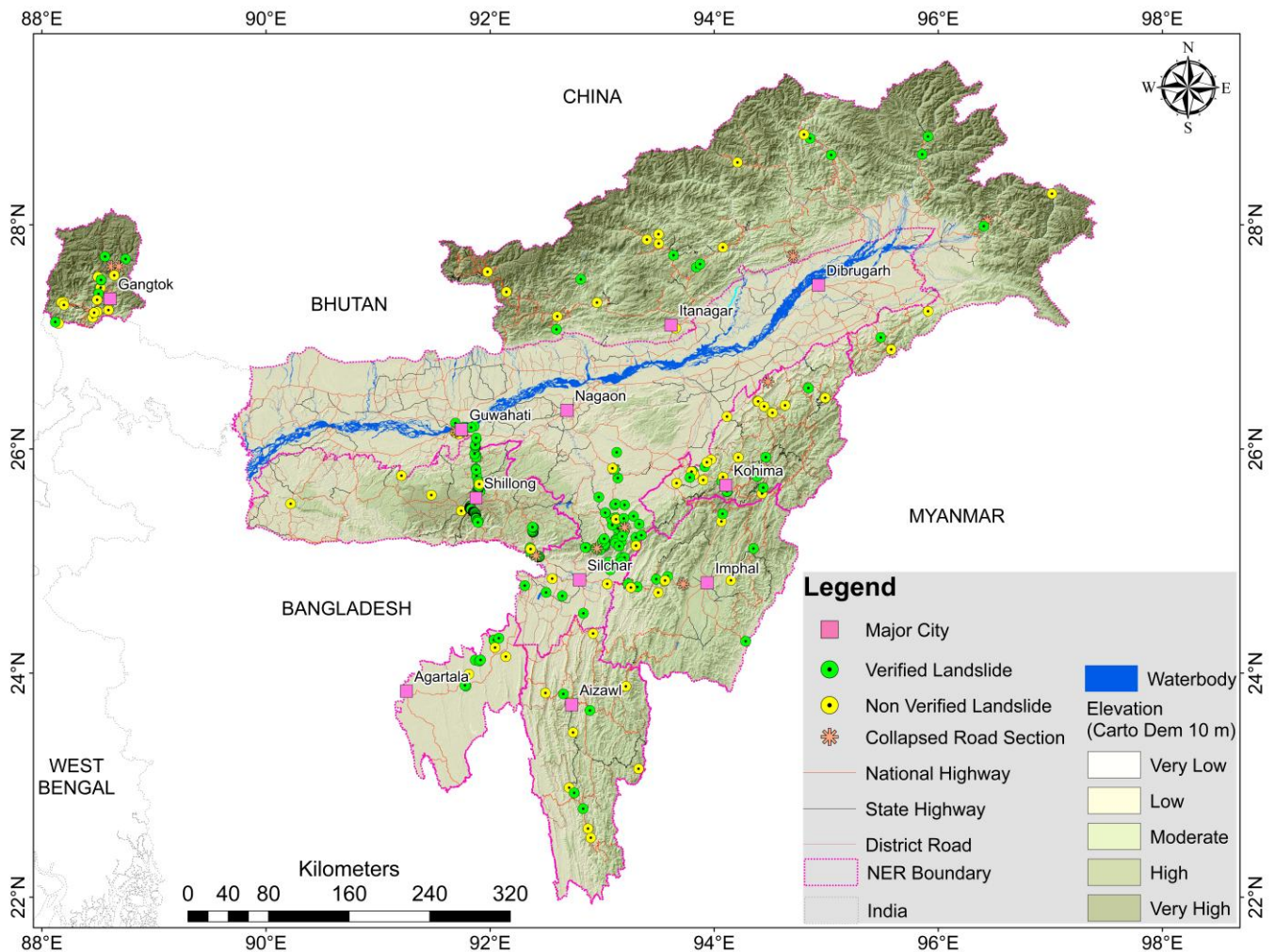
Map 1 Landslide Incidents in the NER, 2025
