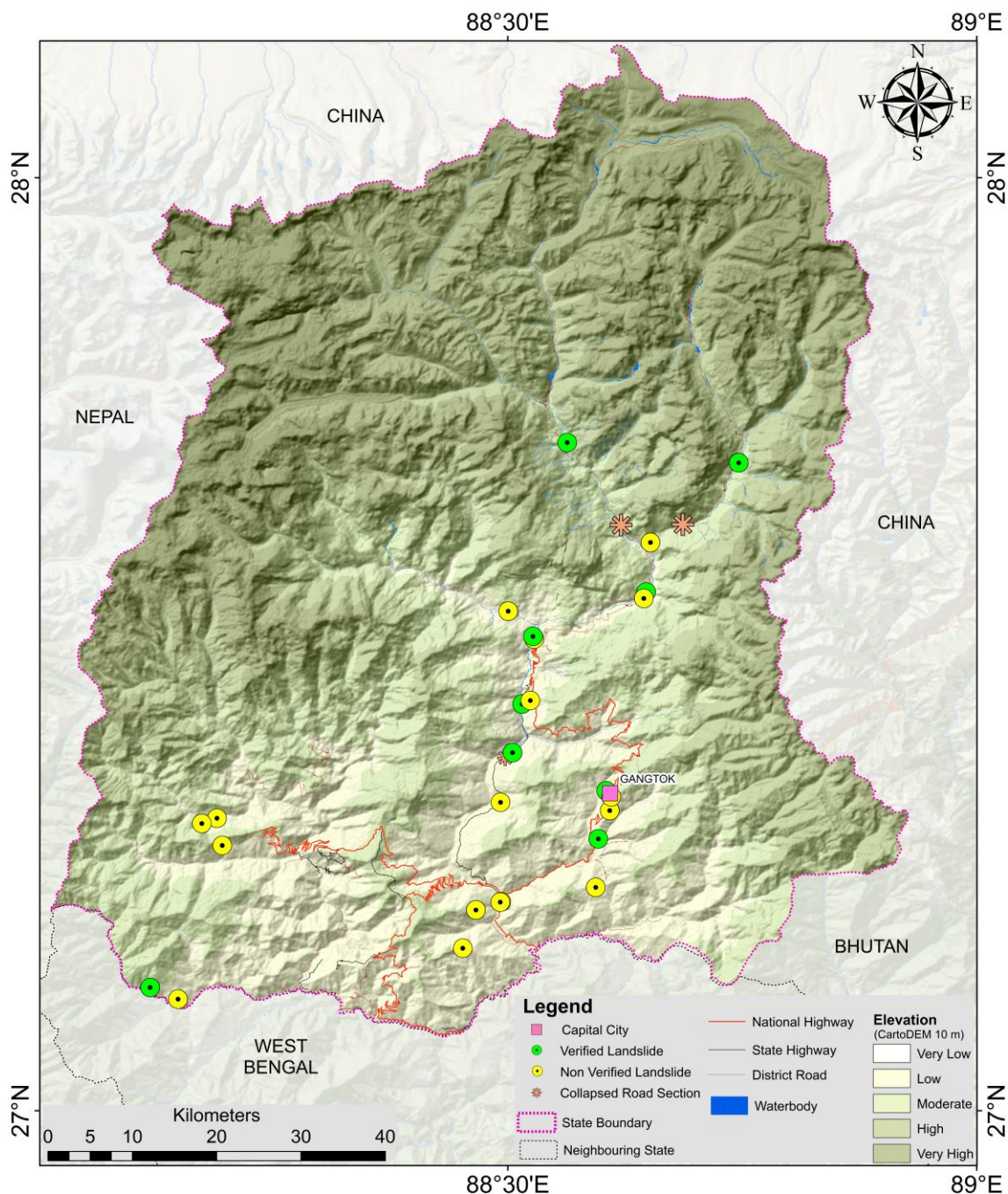
Map 8 Landslide incidents in Sikkim, 2025
