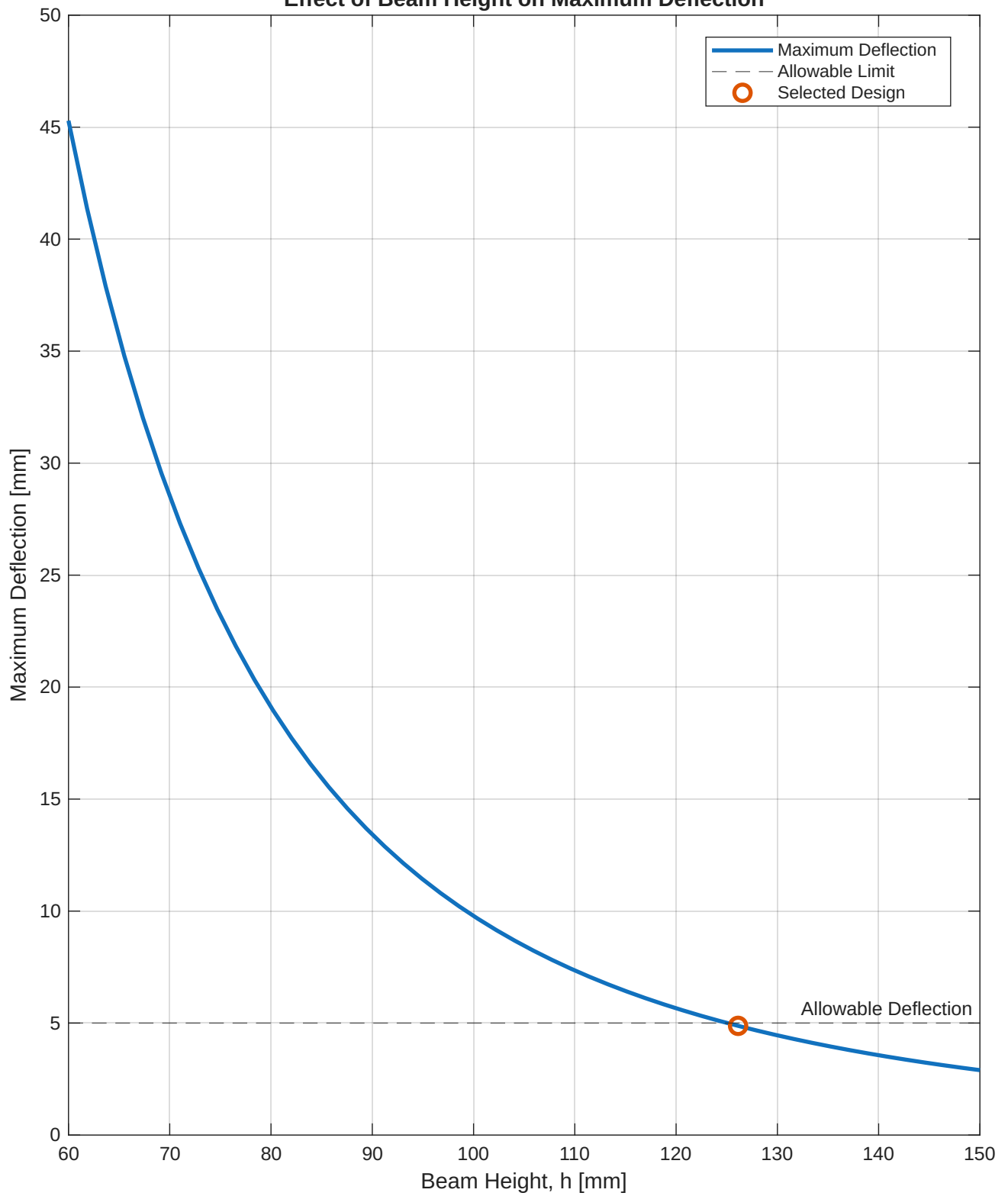
Effect of Beam Height on Maximum Deflection
