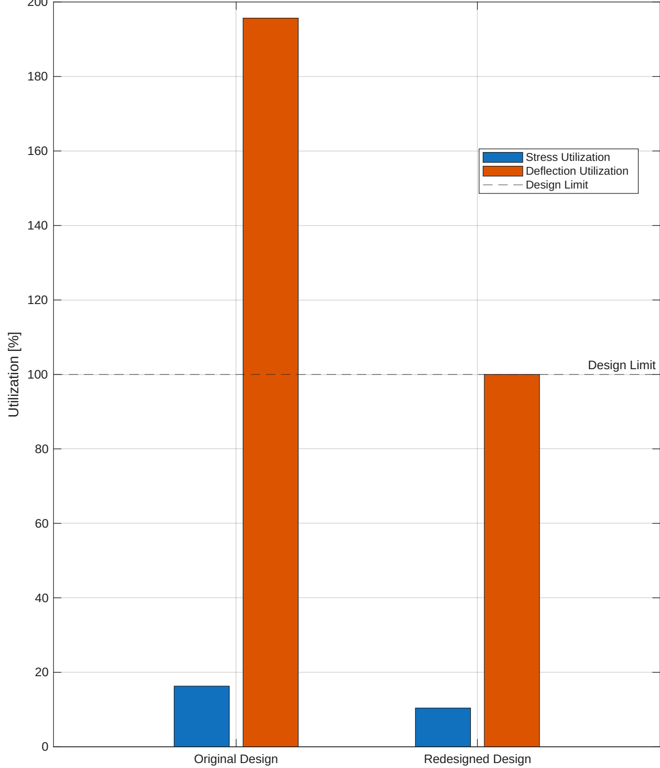
Original vs Redesigned Beam Performance
