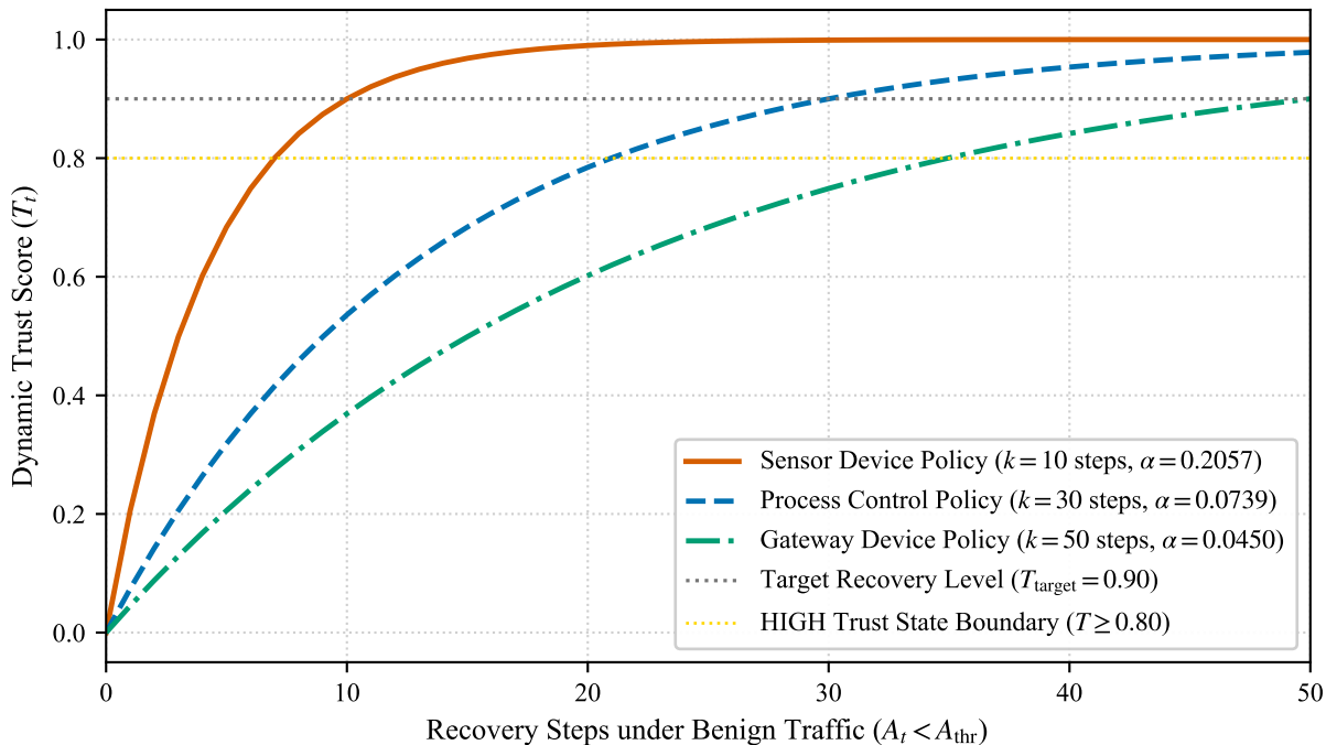
Figure 6: Policy-Parameterized Asymptotic Trust Recovery Curves
