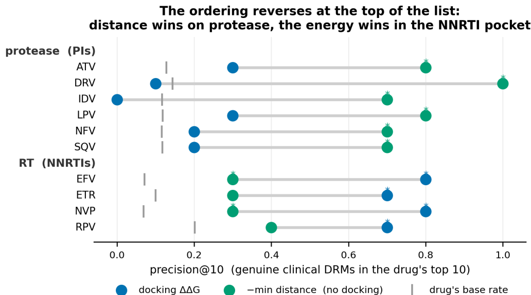
Figure 2: Top of the list, per drug. Precision@10 for the two structure-only predictors, the depth at which the tool is actually read; Table 4 ranks the whole panel instead. Each line joins one drug’s two values, the tick is its DRM base rate, and * marks p < 0.05 by an exact one-sided hypergeometric test against that rate (scripts/15_geometry_baseline.py). The ordering reverses between targets, which is the one place the energy step earns its cost.
