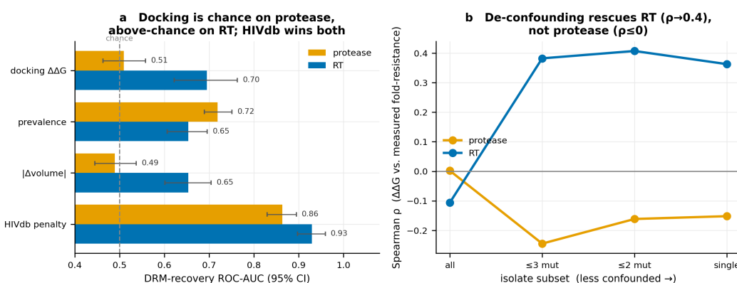
Figure 4: Docking \Delta\Delta G across the two targets. (a) DRM-recovery ROC-AUC with bootstrap 95% CIs: docking- \Delta\Delta G sits on the chance line for protease (0.51) and above it for RT (0.70), but a docking-free ligand-distance baseline beats it on both (Table 5), and the HIVdb expert system wins both. (b) De-confounding: as the fold-resistance target is rebuilt from progressively less co-mutated isolates, RT’s magnitude correlation climbs to \rho \approx 0.4 while protease stays \leq 0 .
