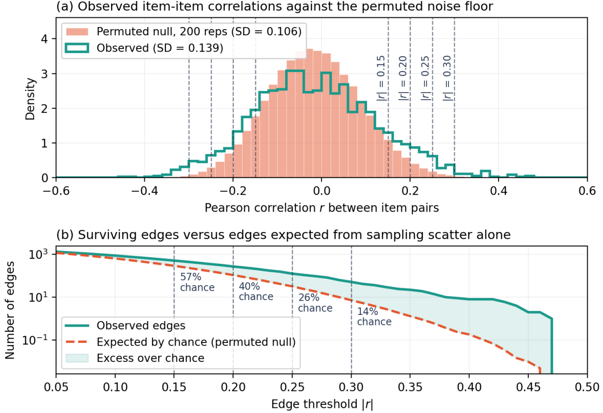
Figure 6: Graph 4. (a) Observed item-item correlations against a 200-replicate permutation null that re-runs the whole pipeline on independently shuffled columns; observed SD 0.139 against 0.106 for the null, with the excess confined to the tails. (b) Surviving edges against edges expected from sampling scatter alone, log scale; the shaded band is the excess over chance. At |r| > 0.15 more than half of surviving edges are chance.
