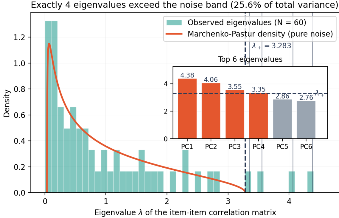
Figure 7: Graph 5. Eigenvalue spectrum of the row-centred item correlation matrix against the Marchenko-Pastur density for pure noise of the same shape ( T = 91 , N = 60 , Q = 1.517 ). The bulk tracks the theoretical curve; exactly four eigenvalues exceed \lambda_+ = 3.283 , carrying 25.6% of total variance. Inset: the top six eigenvalues, showing a clear gap between the fourth (3.35) and the fifth (2.86).
