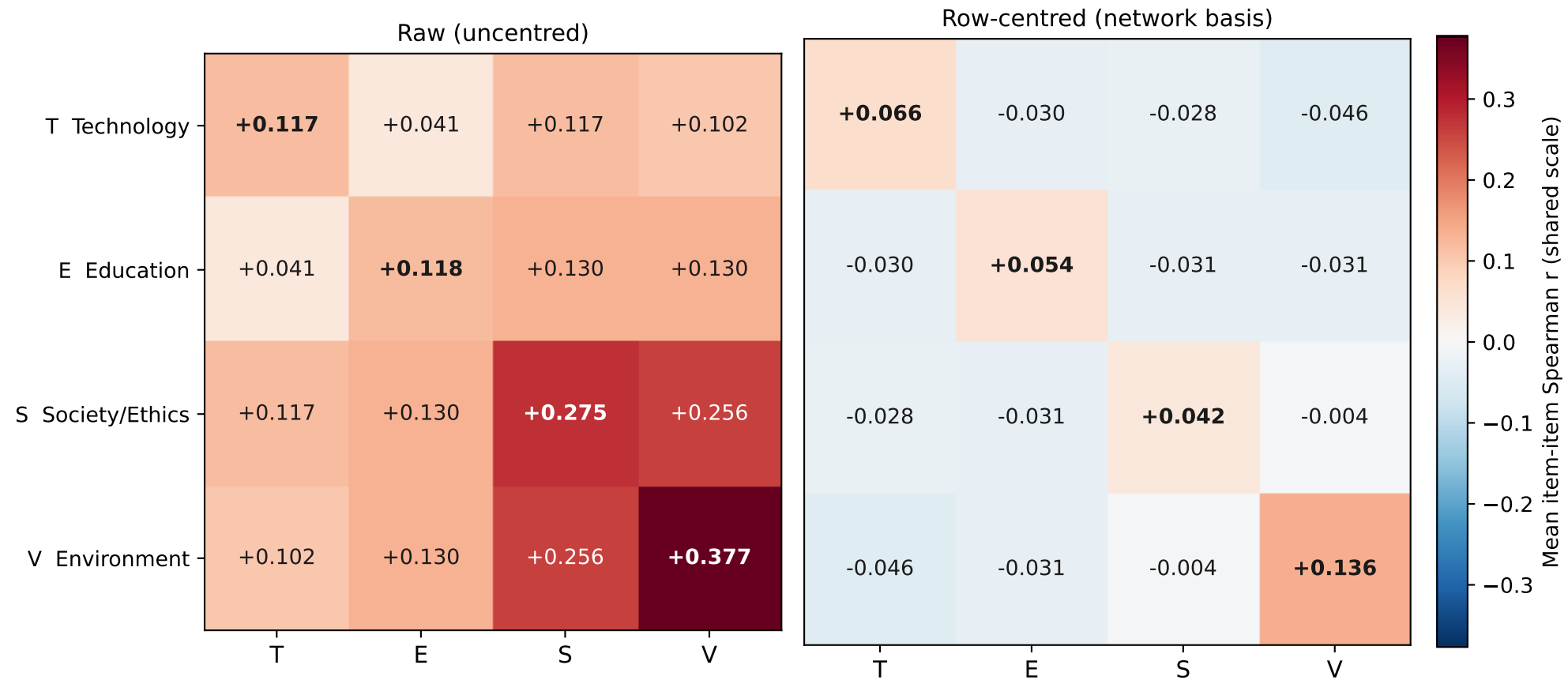
Graph 8: topic-block connectivity, raw vs. row-centred
