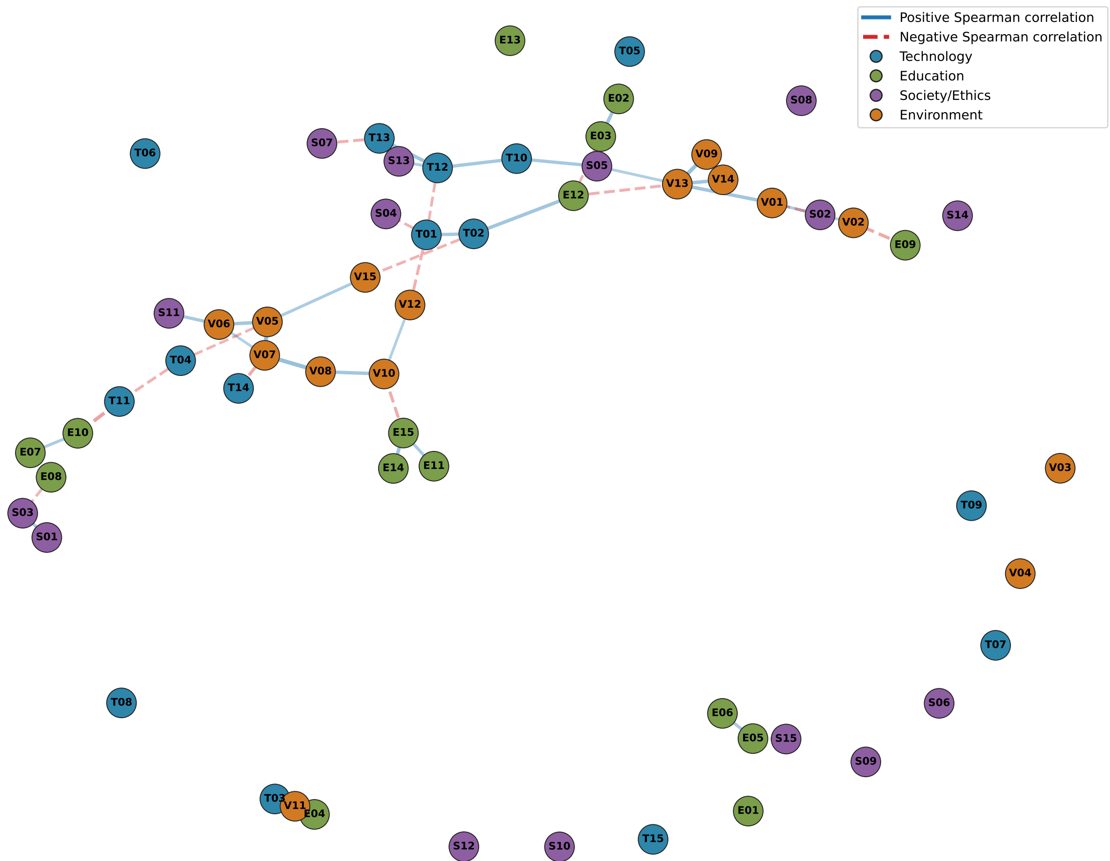
Thresholded questionnaire network (row-centred): |Spearman r | \geq 0.30
