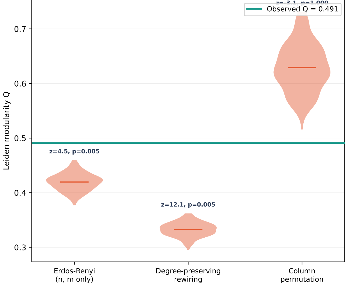
(b) Observed modularity vs three null models Column permutation is the only valid test
