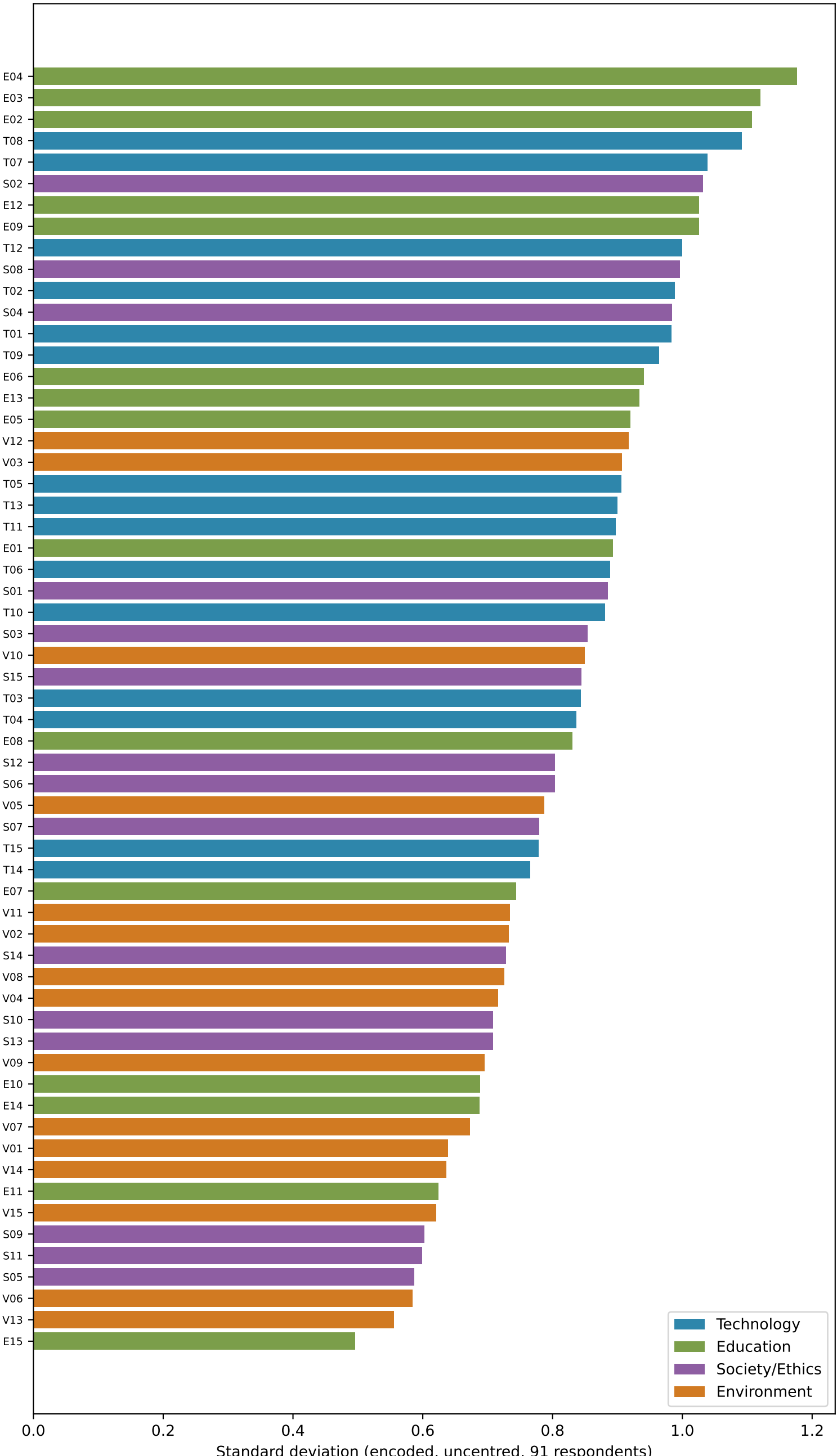
Item variance ranking: contested (top) to consensus (bottom)
