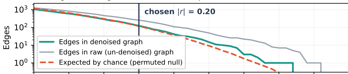
(a) Edge count against the chance expectation
