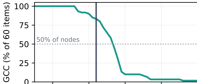
(b) Giant component: where the network shatters
