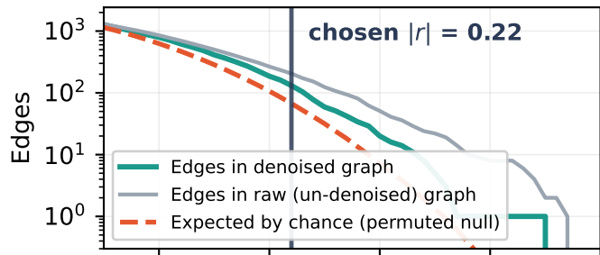
(a) Edge count vs chance expectation
