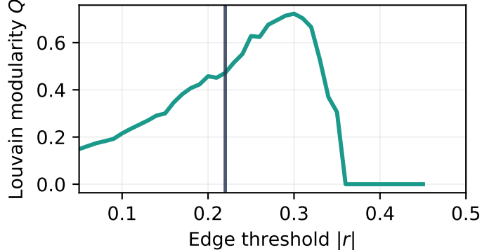
(d) Modularity (rises as the graph fragments)
