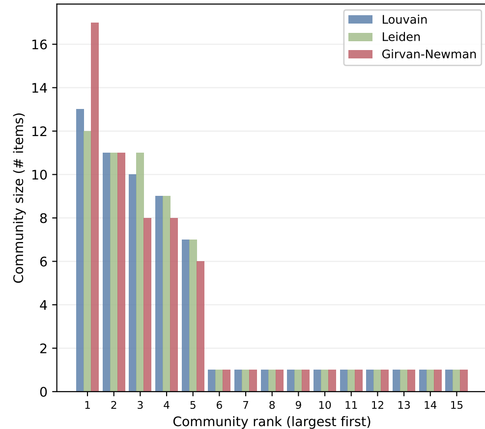
(c) Community size distributions (rank-ordered, 60 items total)
