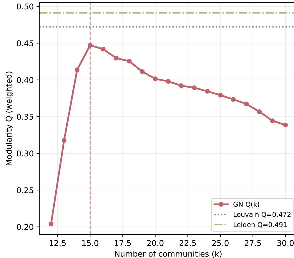
(b) Girvan-Newman Q vs k (dotted = Louvain, dash-dot = Leiden)
