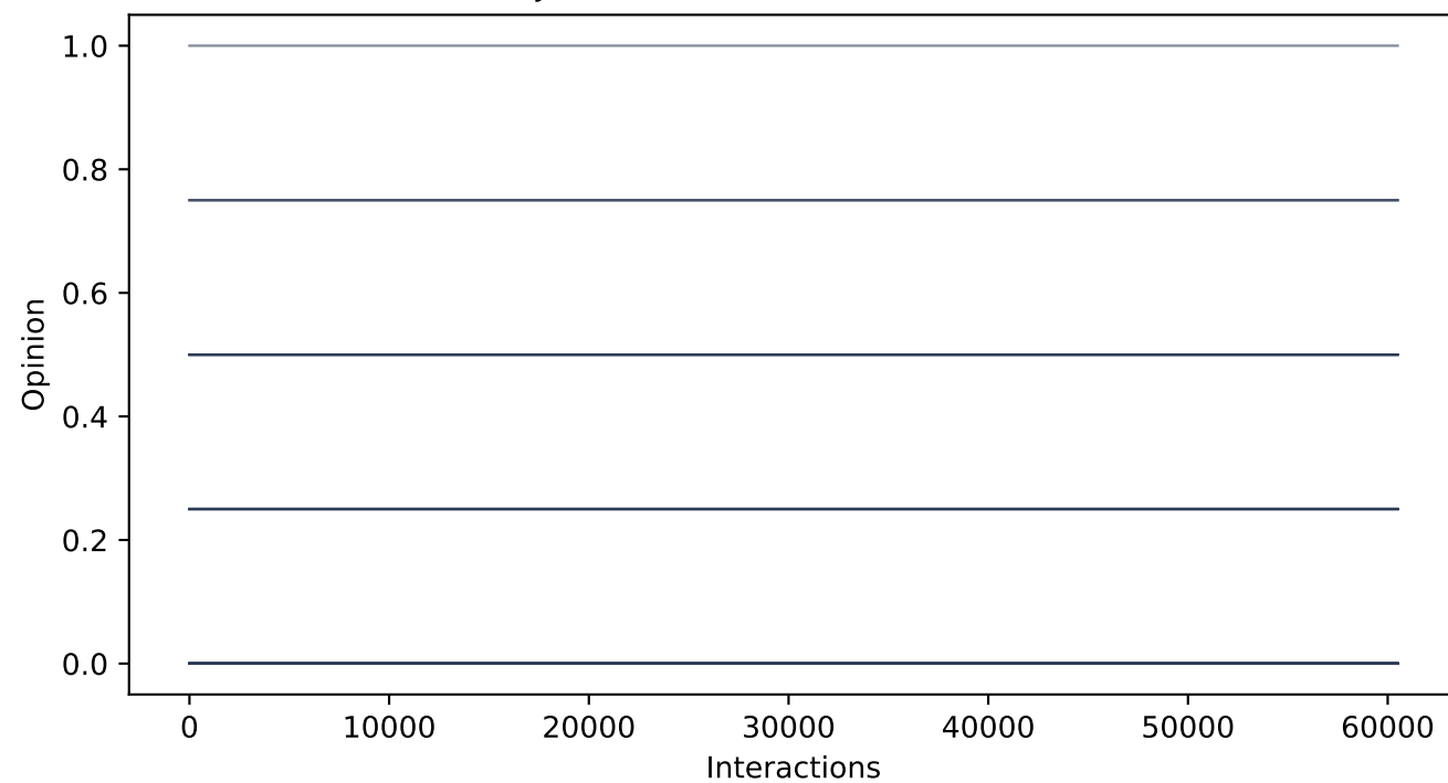
Trajectories at \varepsilon = 0.15 (5 clusters)
