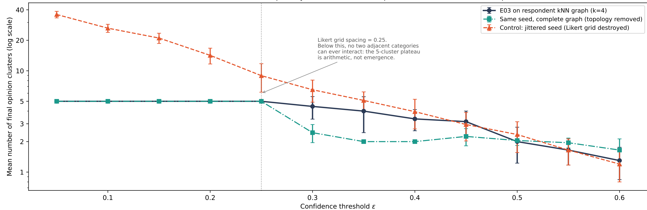
Deffuant-Weisbuch on E03 ("compulsory attendance"), 20 repetitions, 60,000 interactions per run
