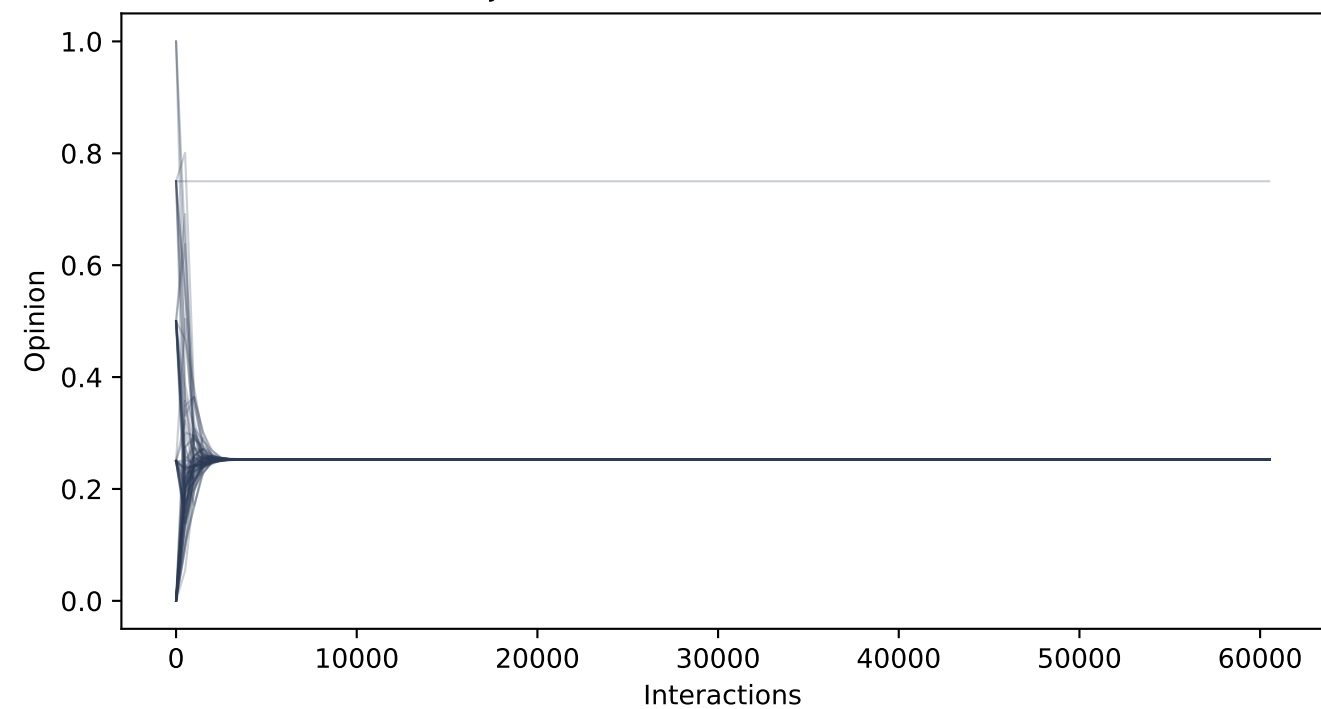
Trajectories at \varepsilon = 0.45 (2 clusters)
