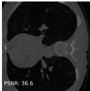
DEFT
