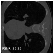
RED-diff
