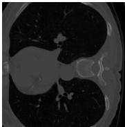
Ground truth
