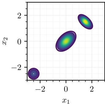
Contour of target \pi
