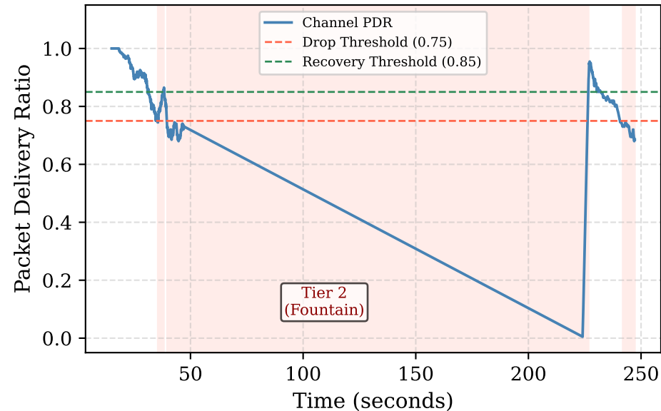
(a) PDR Drop Triggering Tier 2
