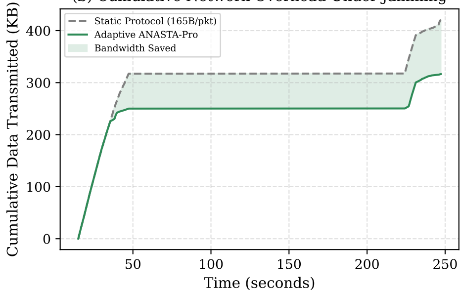
(b) Cumulative Network Overhead Under Jamming
