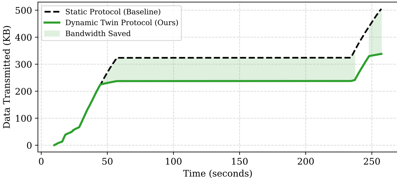
Cumulative Network Overhead Under Jamming
