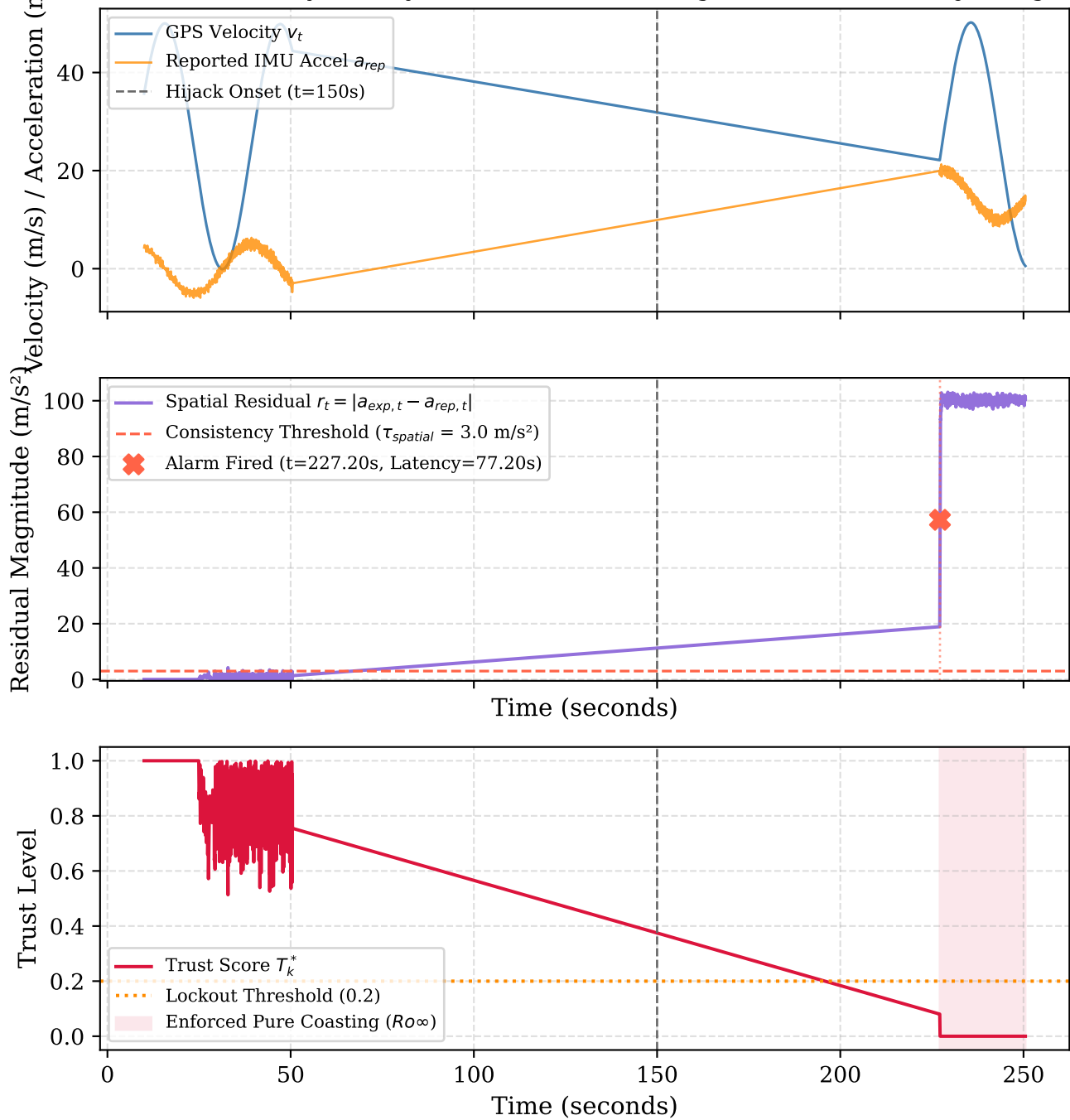
Scenario D: Physics-Layer Cross-Verification Against Transducer Hijacking
