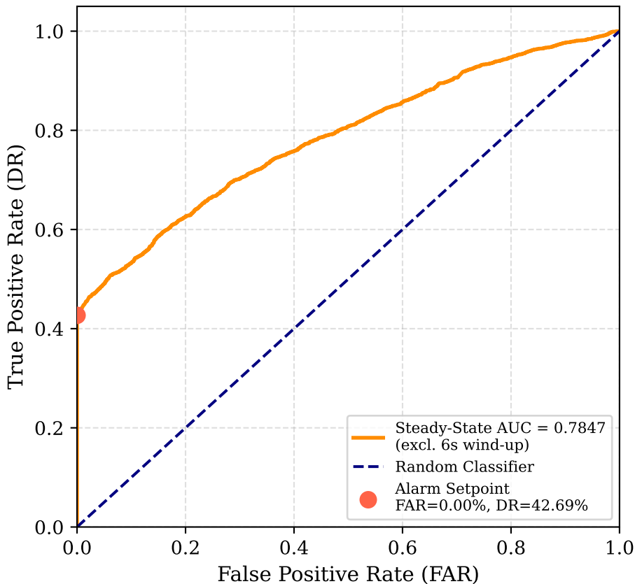
IDS Receiver Operating Characteristic (Steady-State, Stealth Wind-Up Excluded)
