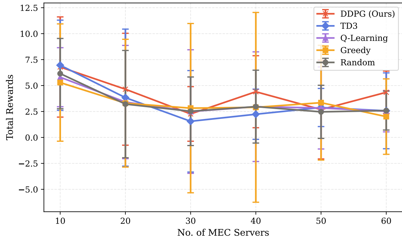
Reward vs. Number of MEC Servers
