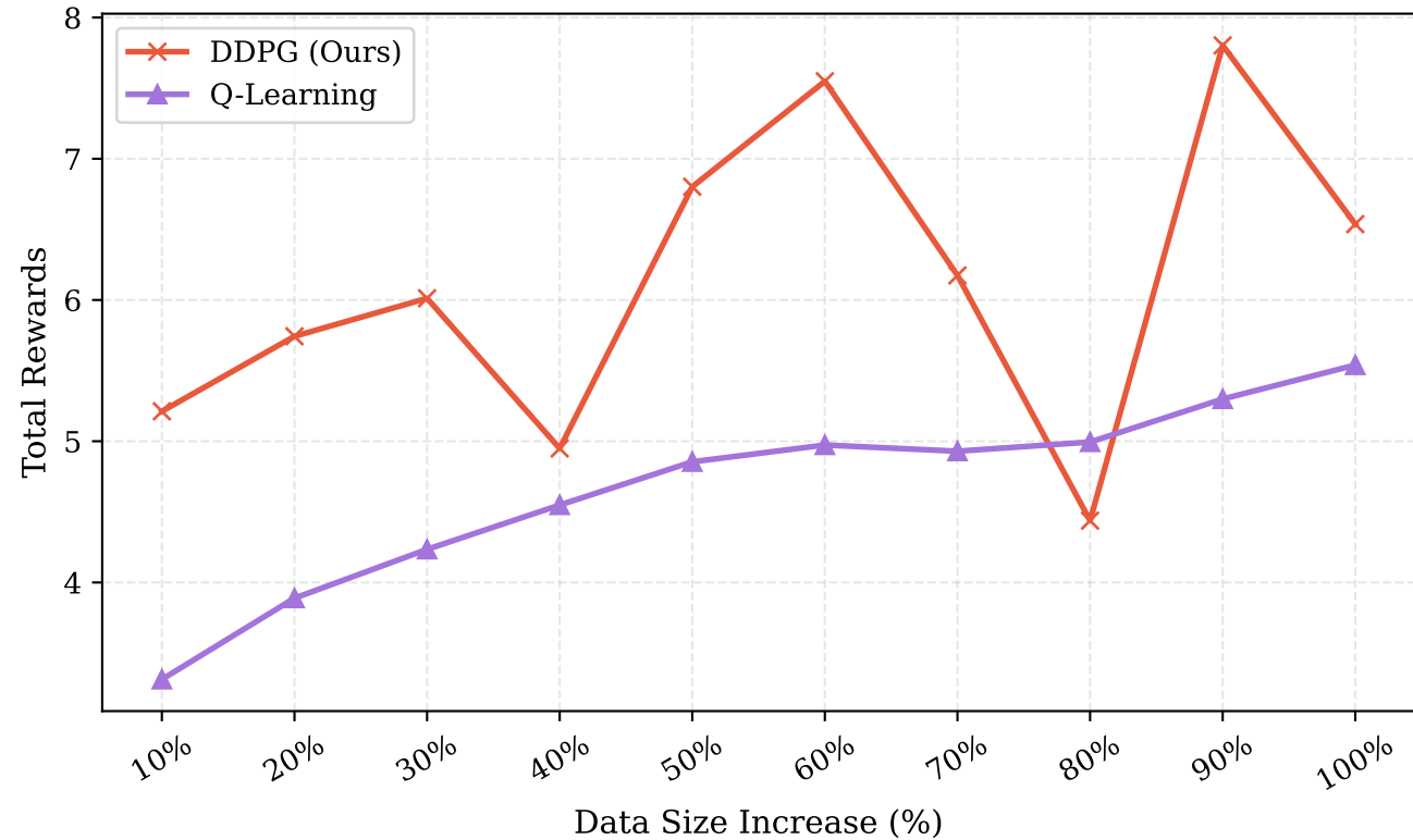
Effect of Data Size on Rewards
