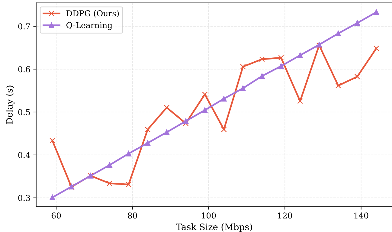
End-to-End Delay: DDPG vs Q-Learning
