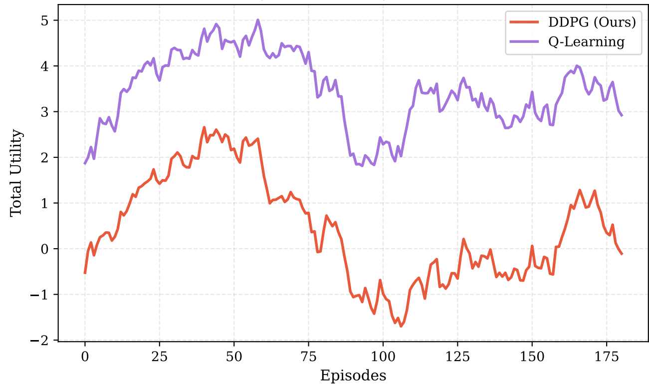
Convergence: Learning Rate \alpha = 0.01
