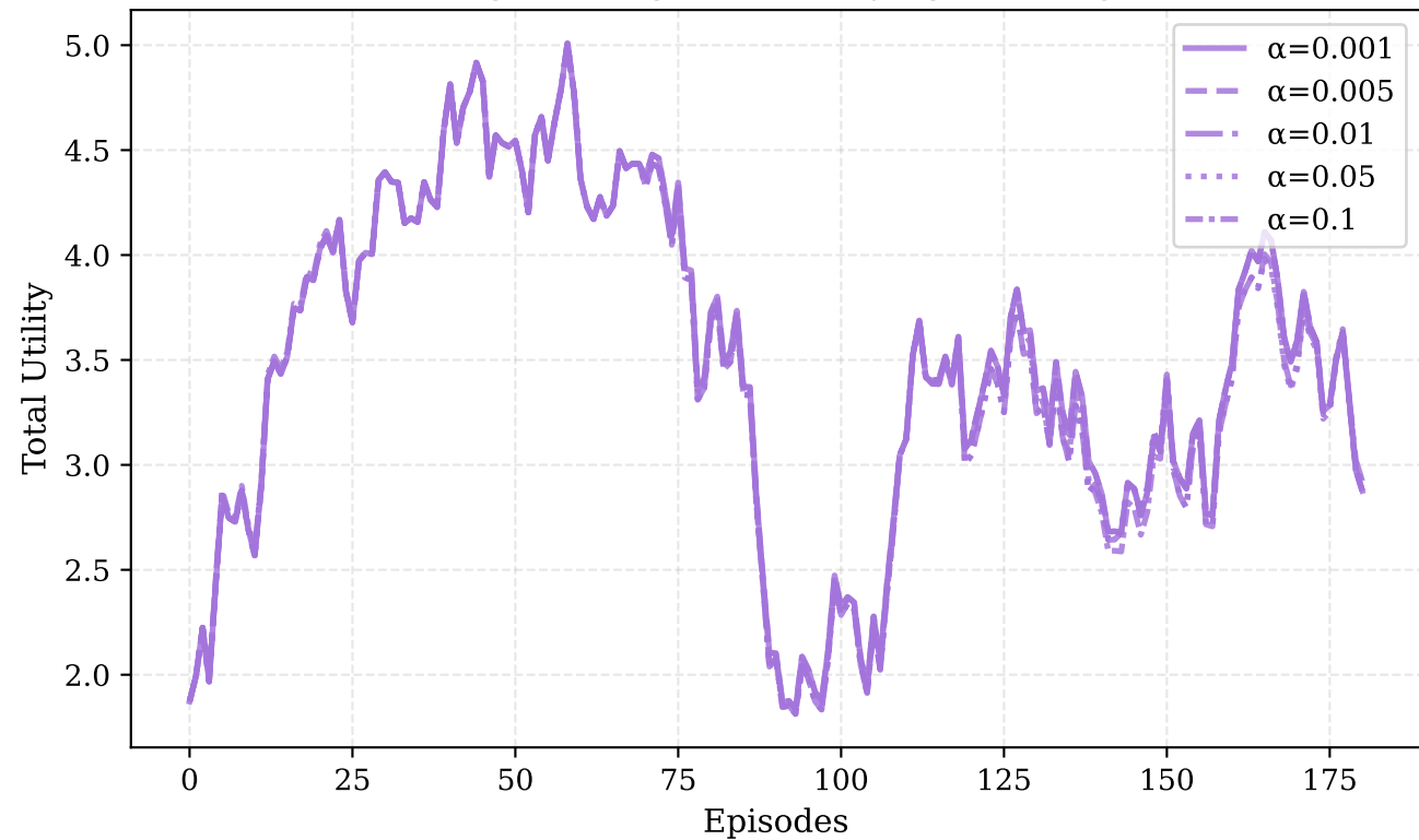
Q-Learning Convergence — Varying Learning Rate \alpha
