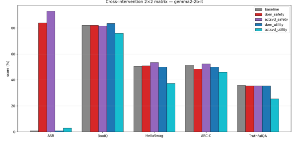
Figure 3: Gemma 2 \times 2 cross-intervention matrix plot corresponding to the results in Section 5.3.
