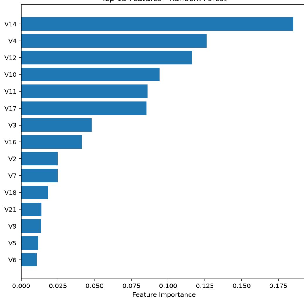
Top 15 Features - Random Forest
