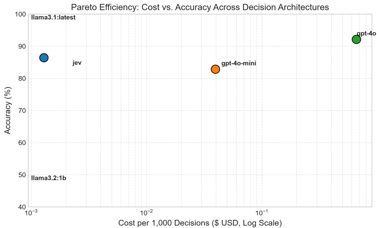
Figure 1: Cost vs. Accuracy Pareto Frontier
