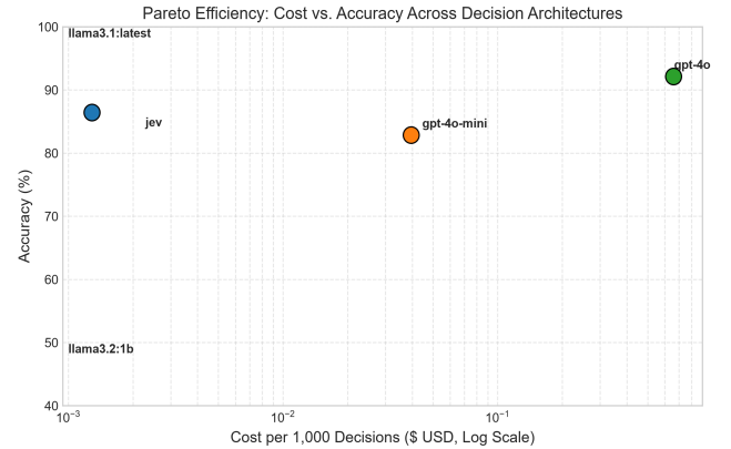
Fig. 1. Cost vs. Accuracy Pareto Frontier across decision architectures.
