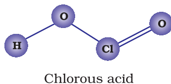
Fig. 7.8 The structures of oxoacids of chlorine
