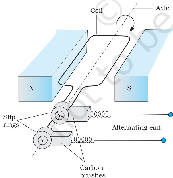
FIGURE 6.13 AC Generator
